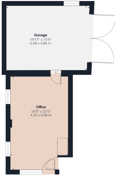
Floor 0 Building 2
